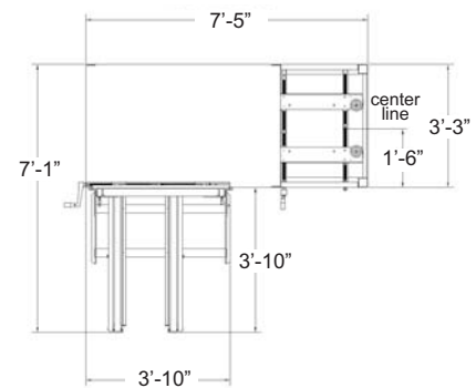
Duraformer 1 right hand layout
