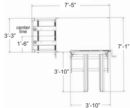
Duraformer 1 left hand layout
